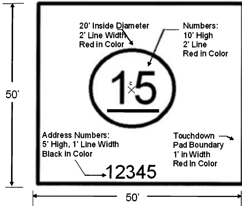
Figure 1108.1.7 Helicopter Landing Pad Markings
