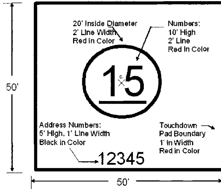
Figure 1108.1.7 Helicopter Landing Pad Markings
